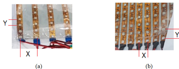
Figure 4: Comparison of LED spacing, (a) Before (unwanted), (b) After (as desired)
