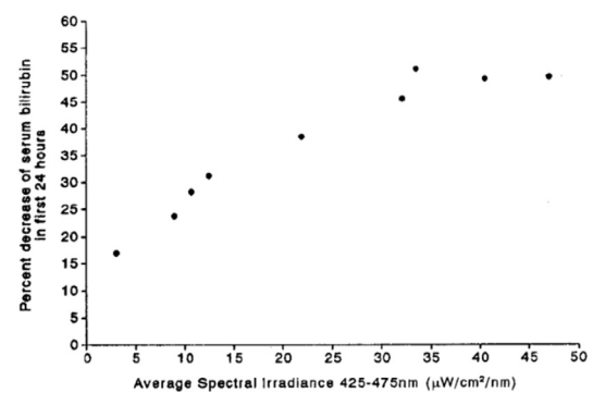
Figure 15: The relationship between the average spectral irradiance and the decrease in serum bilirubin concentration. Term infants with nonhemolytic hyperbilirubinemia were exposed to a special blue light (Phillips TL 52/20W) with different intensities. Spectral irradiance was measured as the average of the head, trunk, and knee readings.
